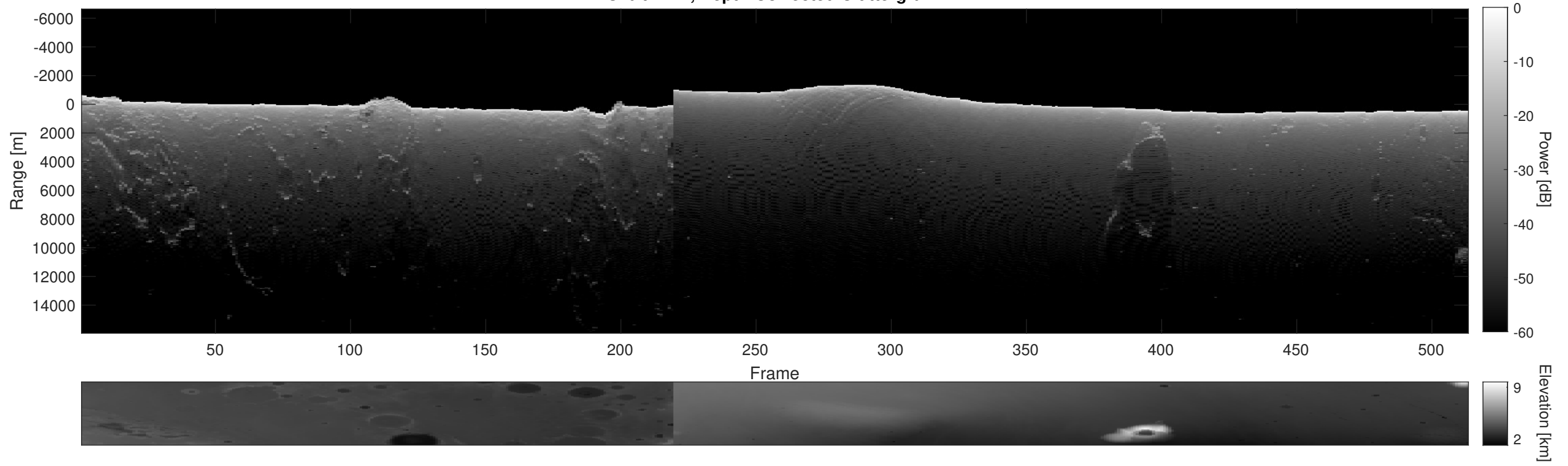
Orbit 4241, Depth-Corrected Cluttergram
