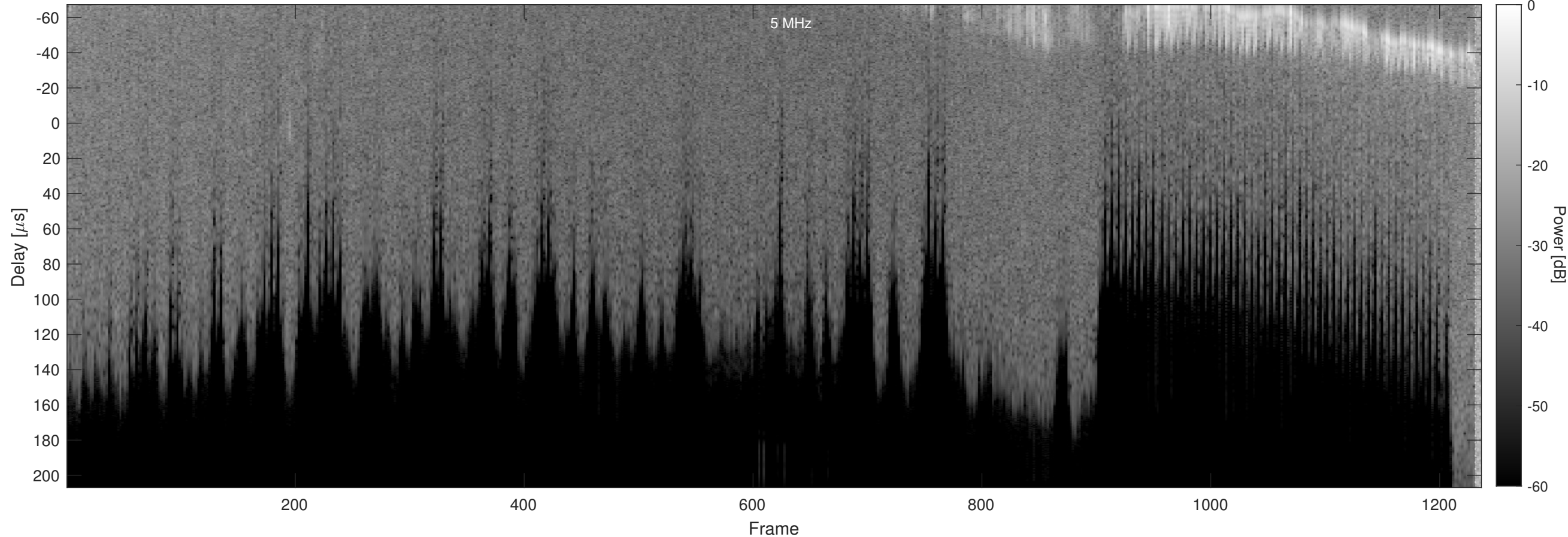
Orbit 4242, Chapman, No Window, Channel 2
