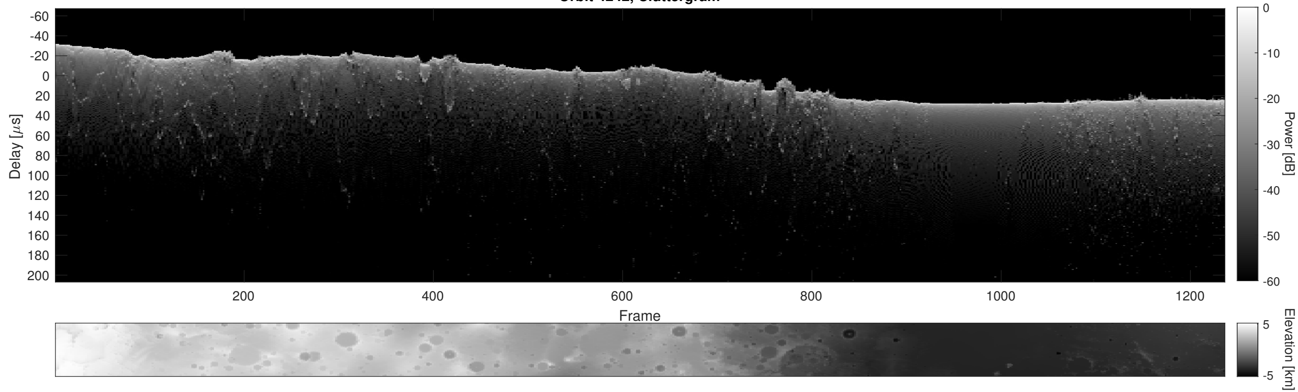
Orbit 4242, Cluttergram
