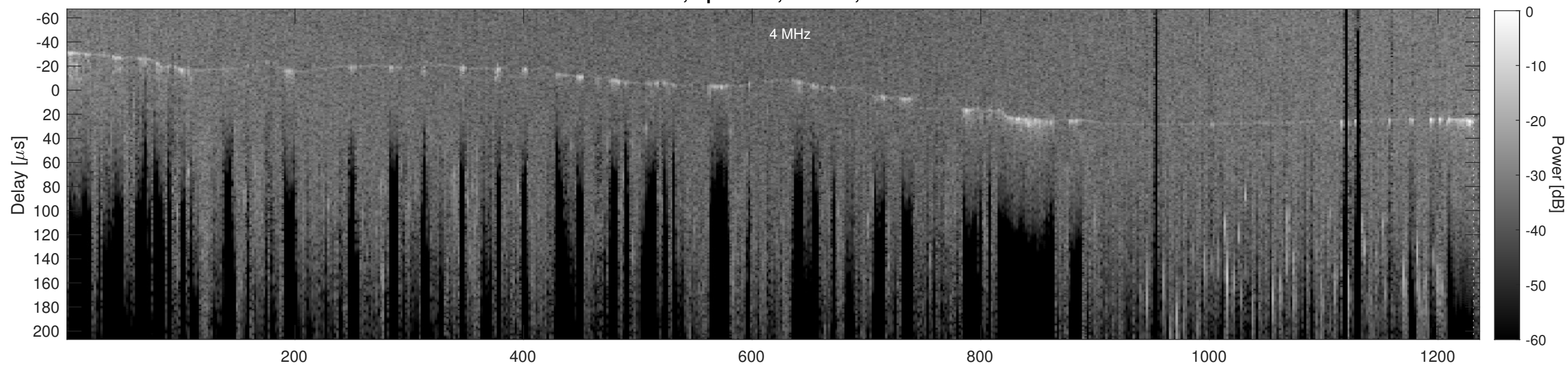
Orbit 4242, Cluttergram
