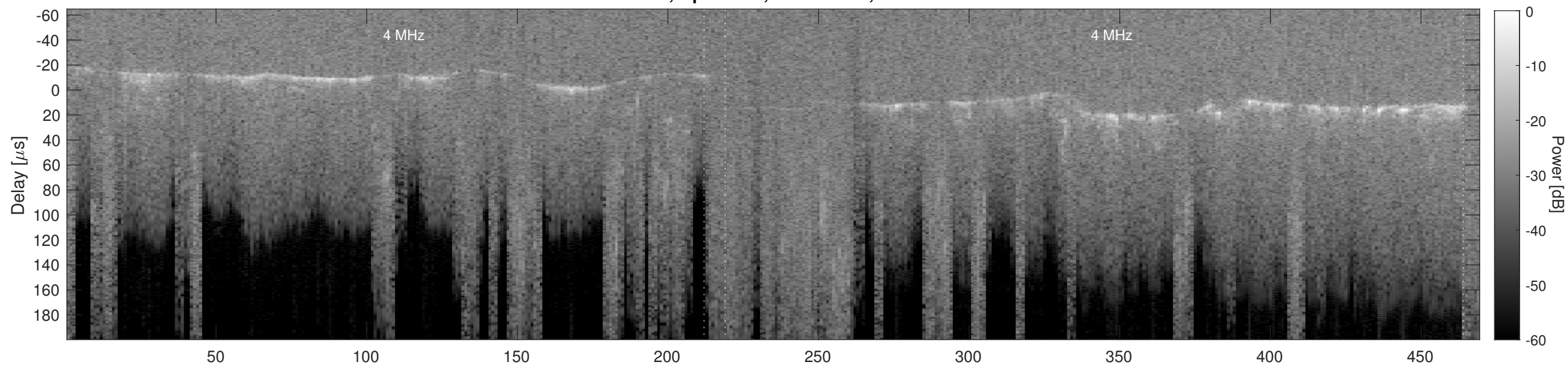
Orbit 4247, Cluttergram
