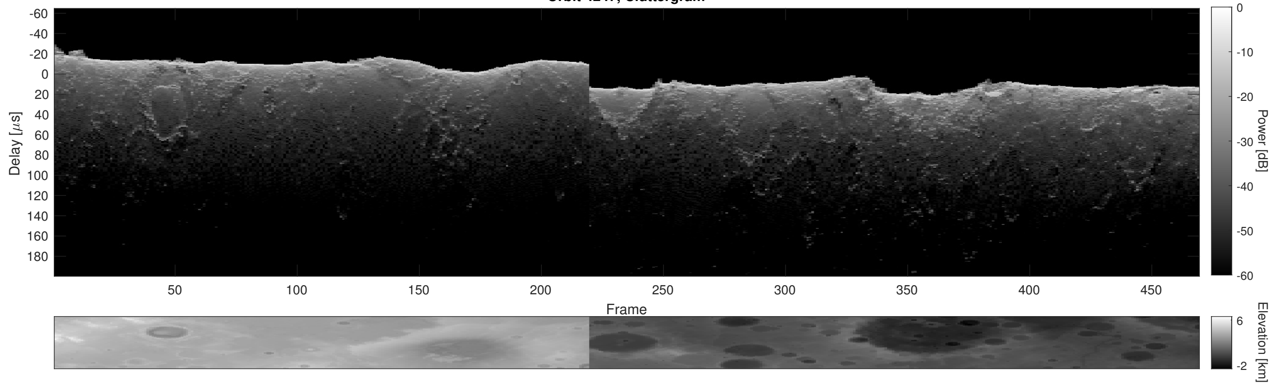
Orbit 4247, Cluttergram
