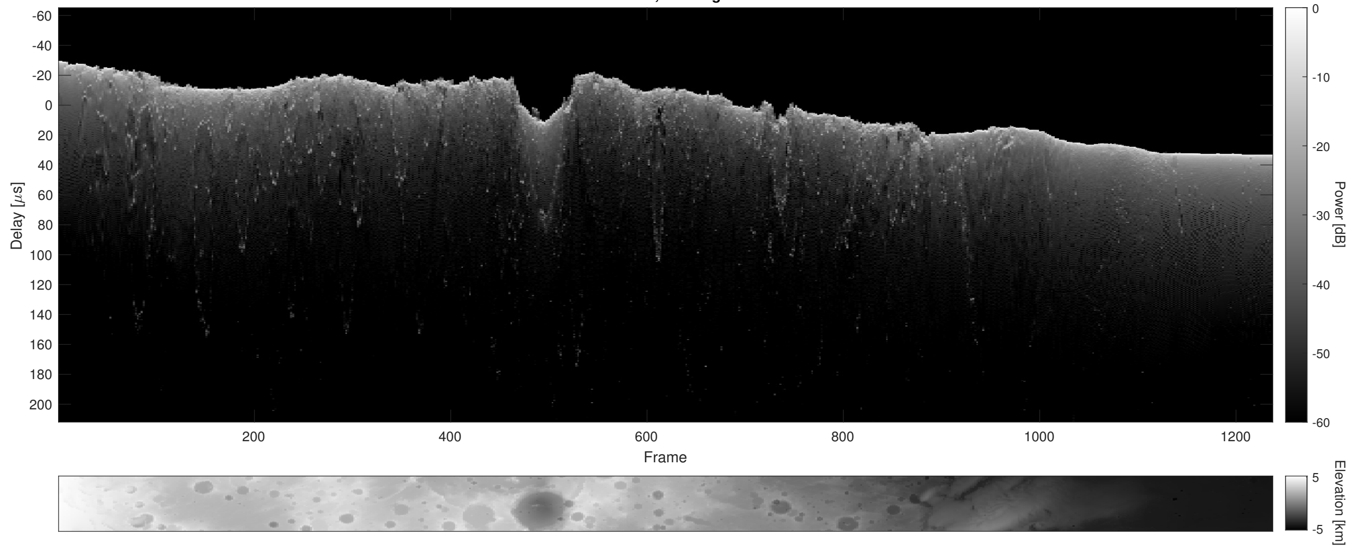
Orbit 4249, Cluttergram
