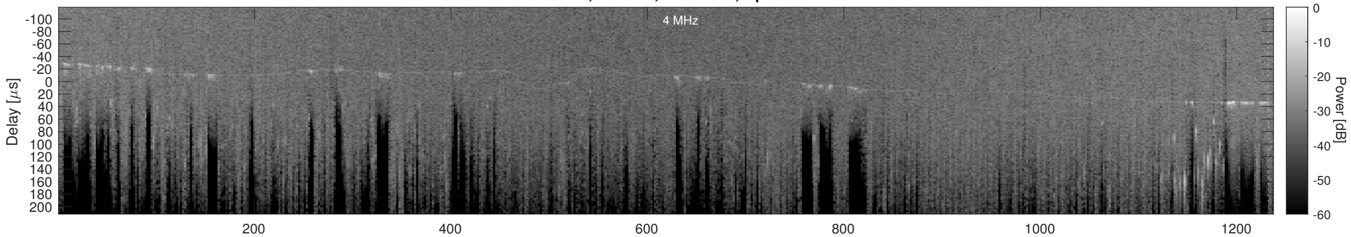
Orbit 4249, Cluttergram
