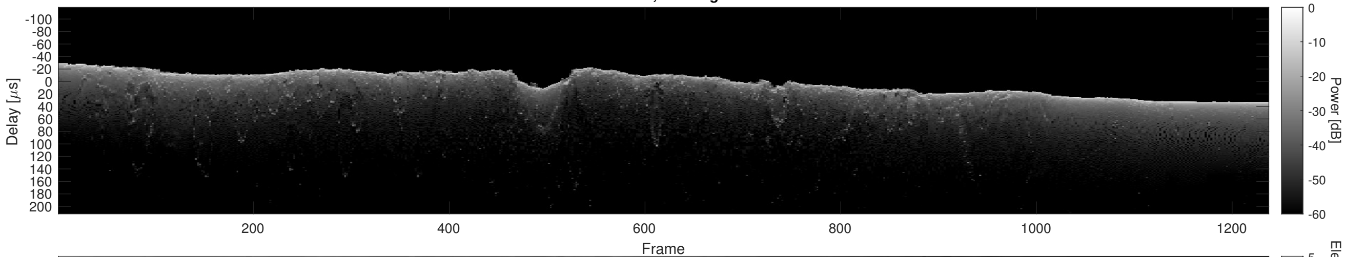
Orbit 4249, Cluttergram
