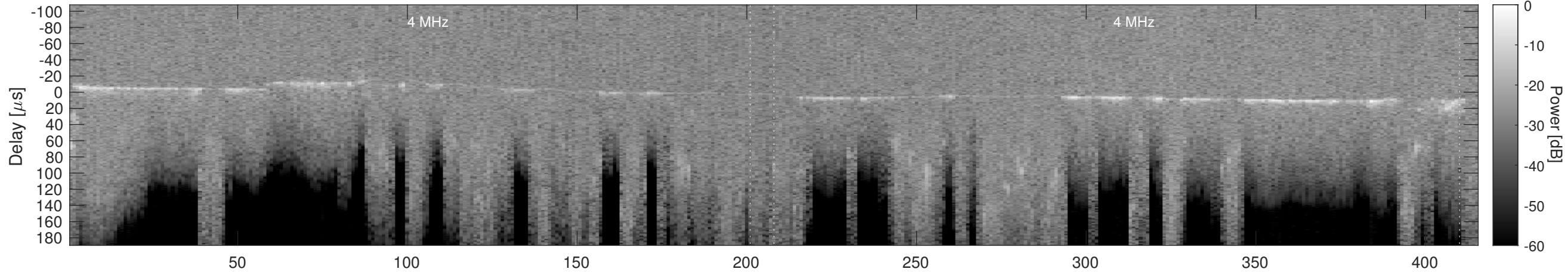
Orbit 4254, Cluttergram
