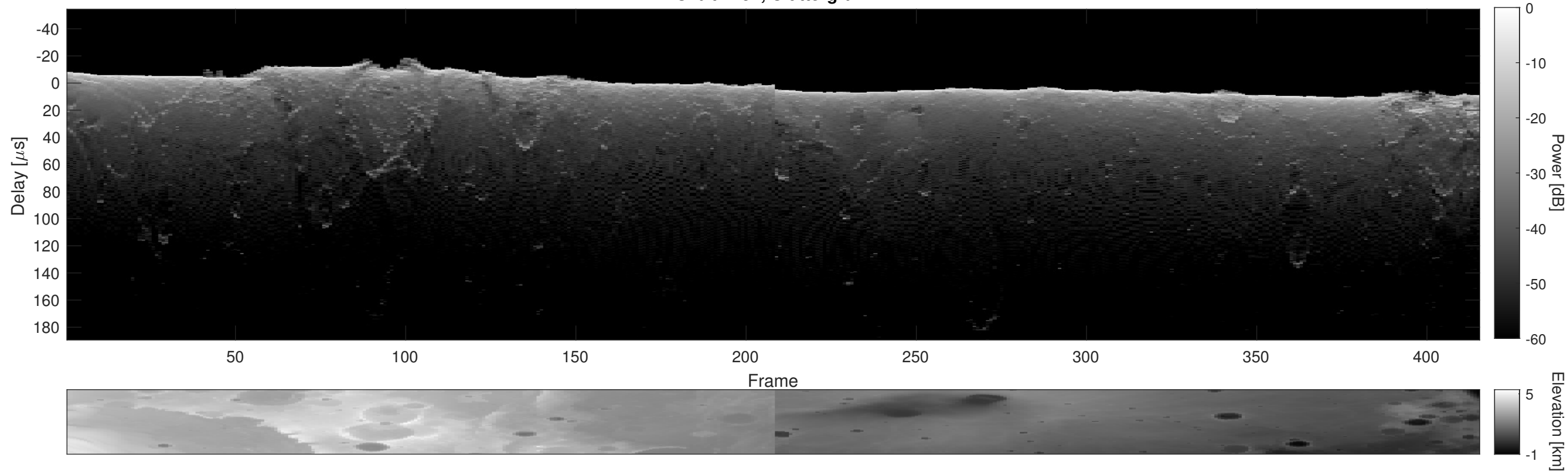
Orbit 4254, Cluttergram
