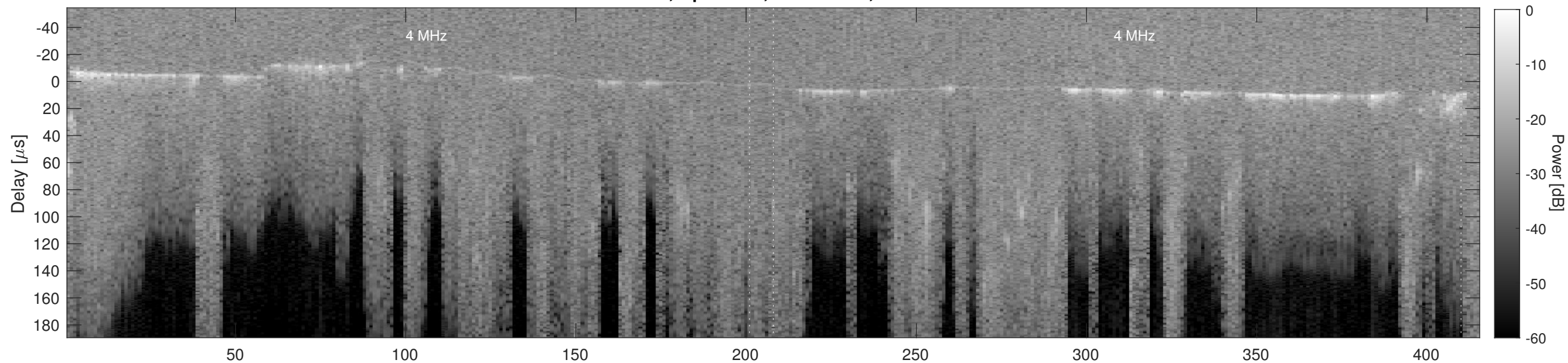
Orbit 4254, Cluttergram
