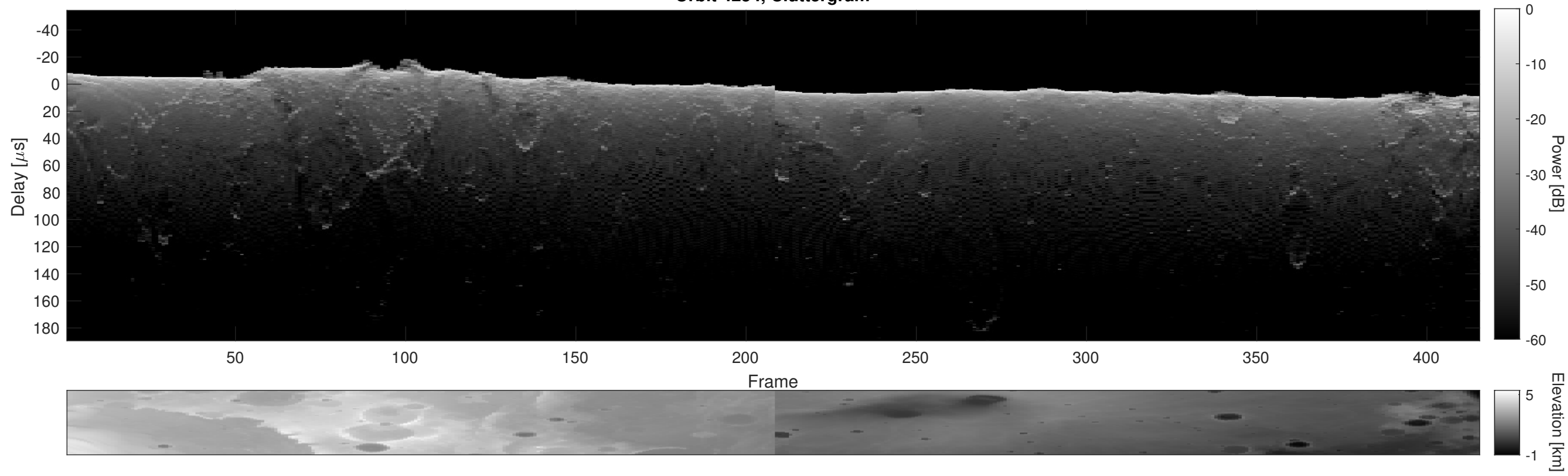
Orbit 4254, Cluttergram
