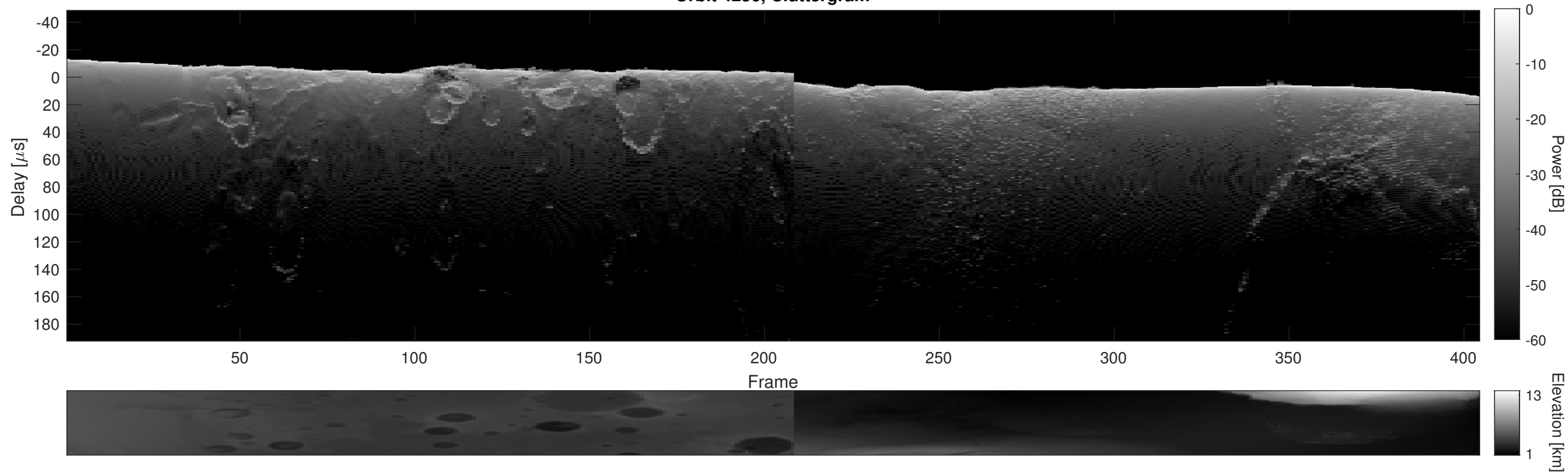
Orbit 4256, Cluttergram
