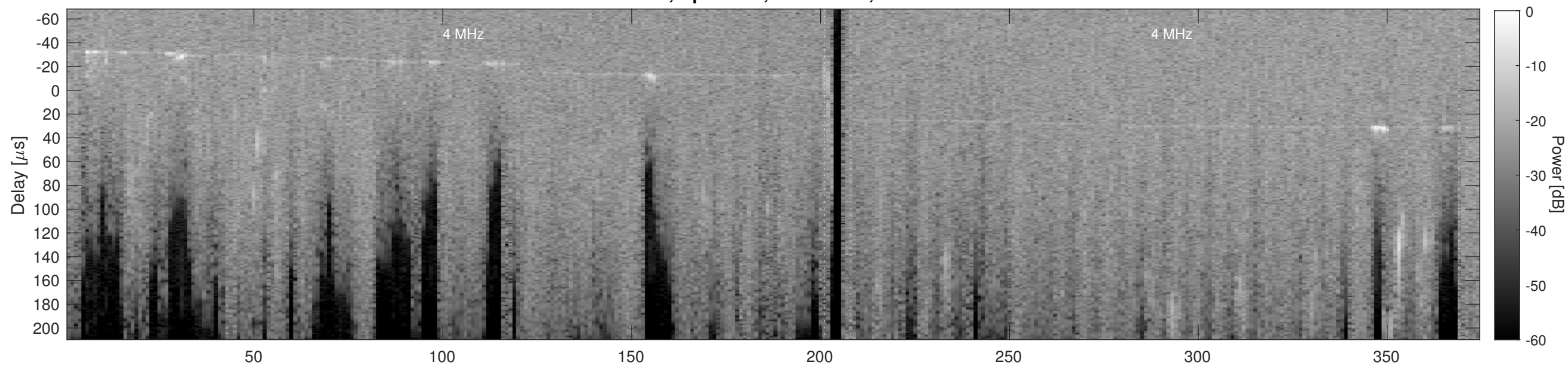
Orbit 4260, Cluttergram
