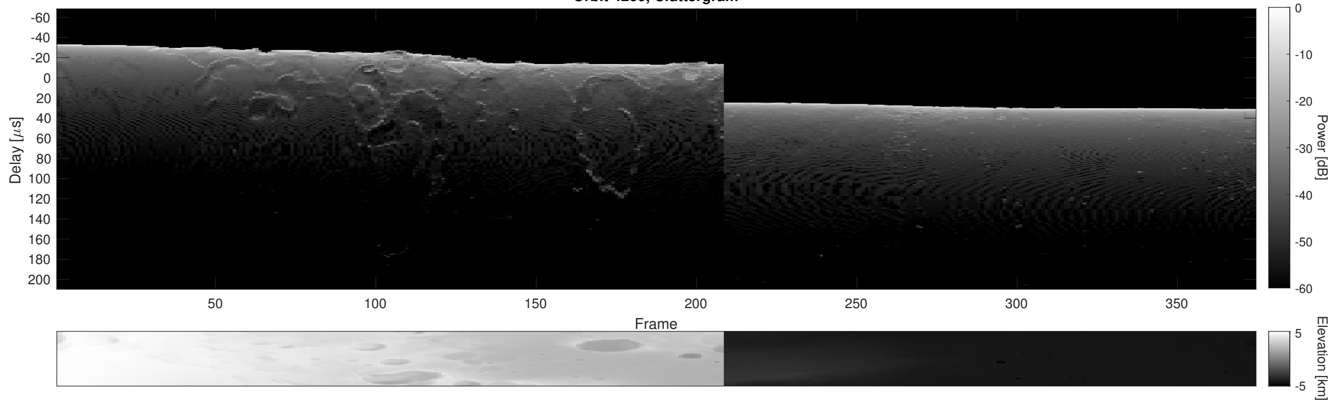
Orbit 4260, Cluttergram
