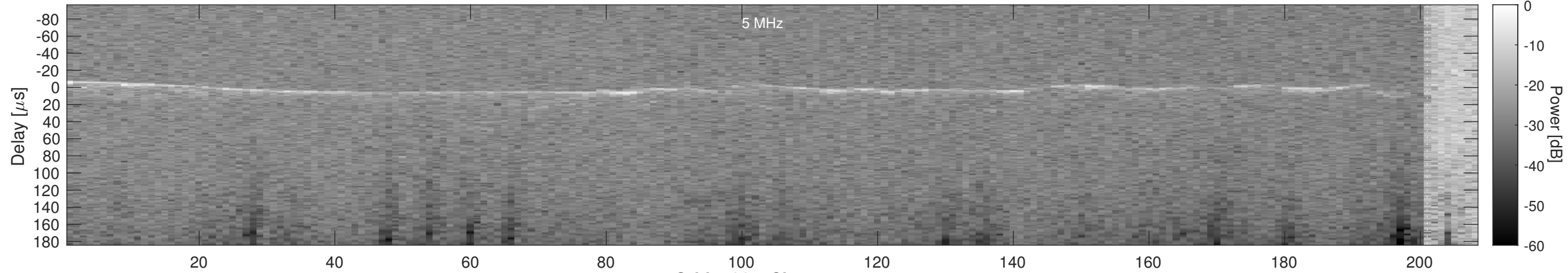
Orbit 4261, Cluttergram
