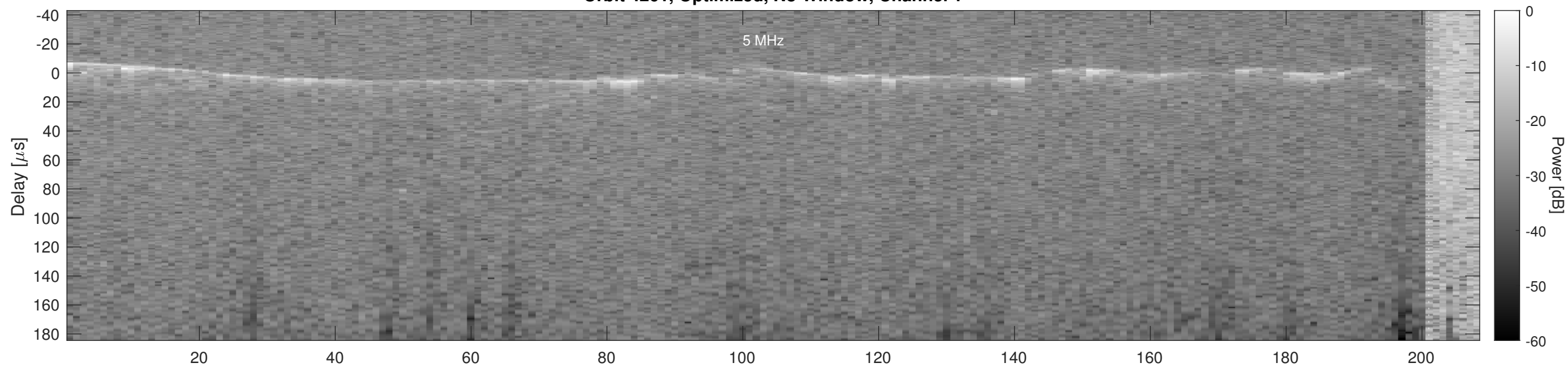
Orbit 4261, Optimized, No Window, Channel 2
