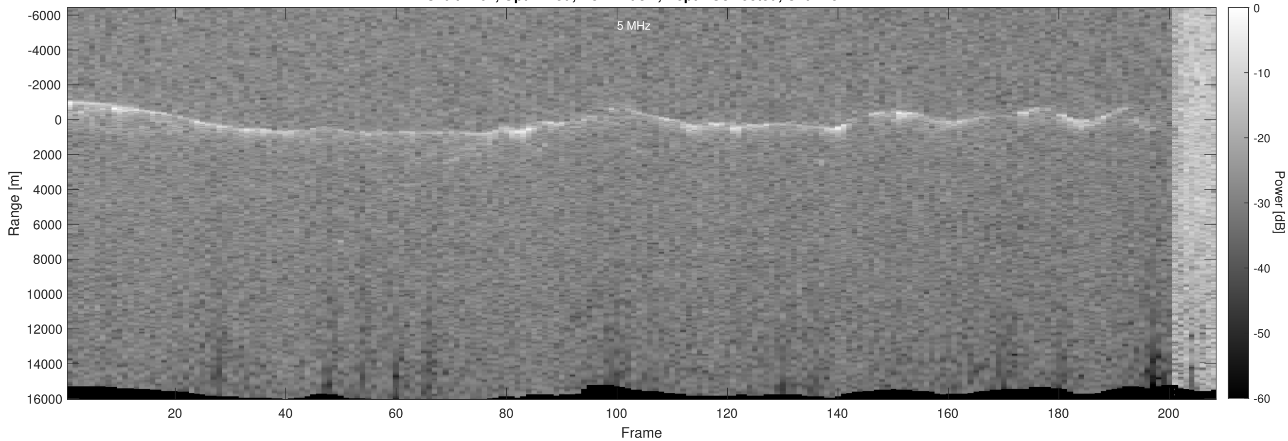
Orbit 4261, Optimized, No Window, Depth-Corrected, Channel 2
