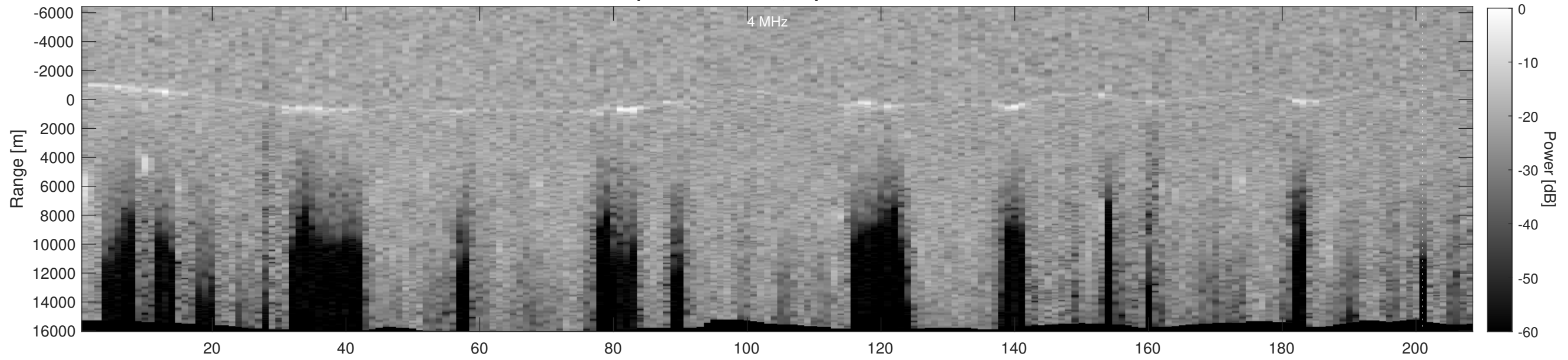
Orbit 4261, Depth-Corrected Cluttergram
