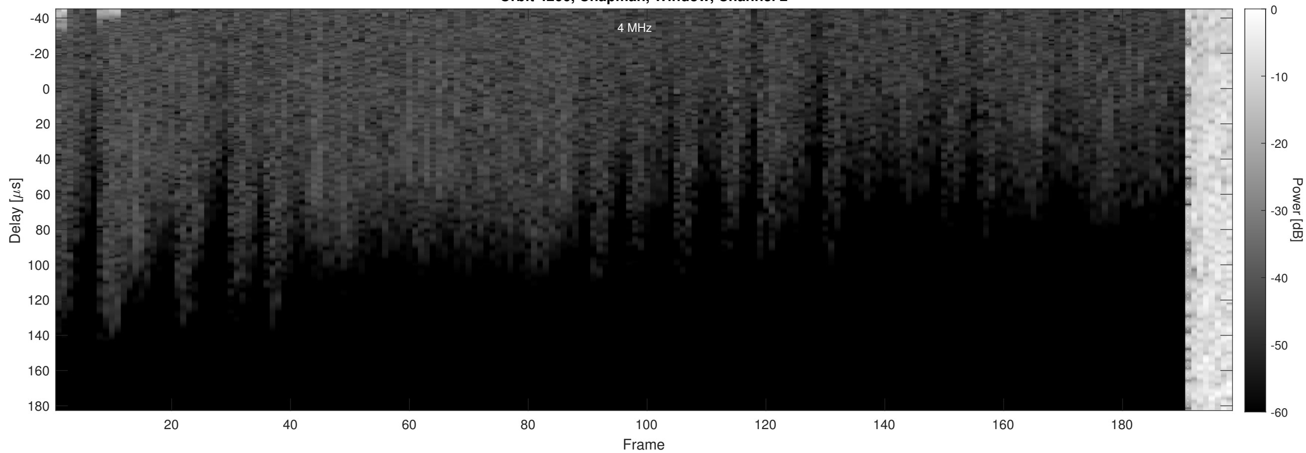
Orbit 4266, Chapman, Window, Channel 2
