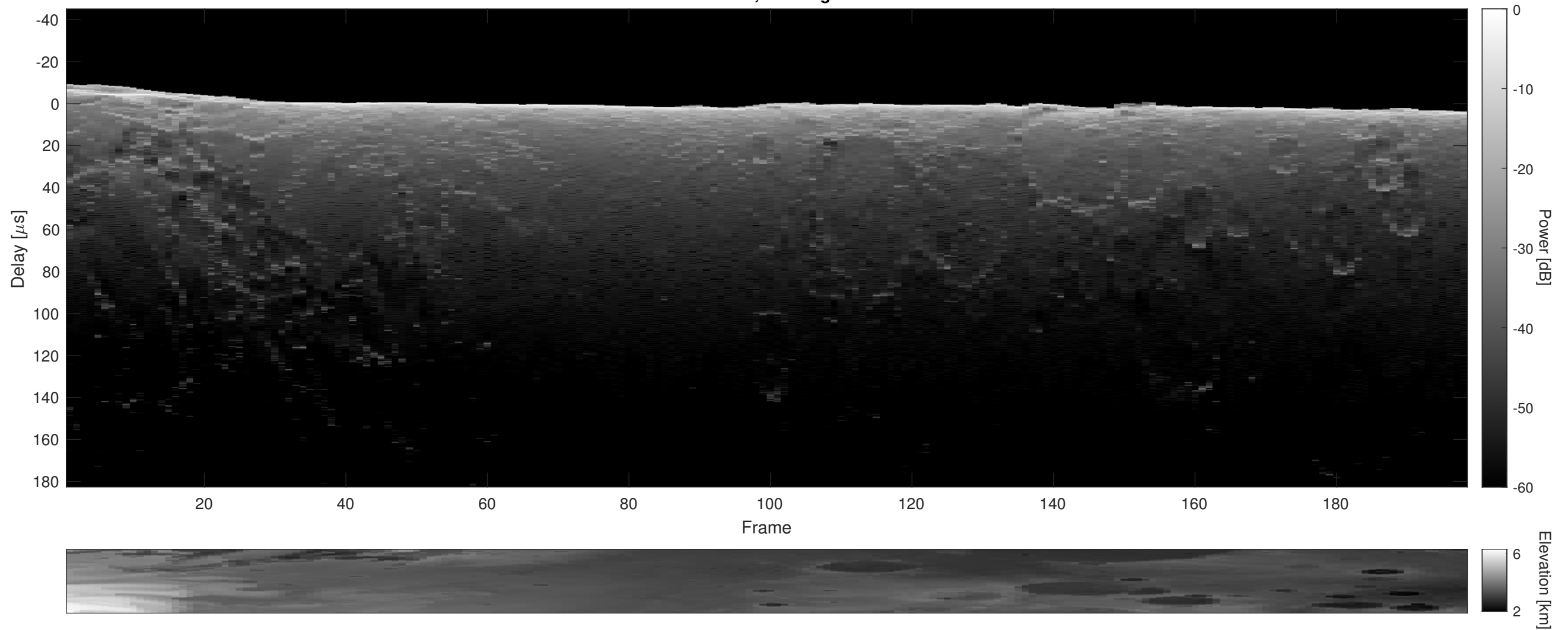
Orbit 4266, Cluttergram
