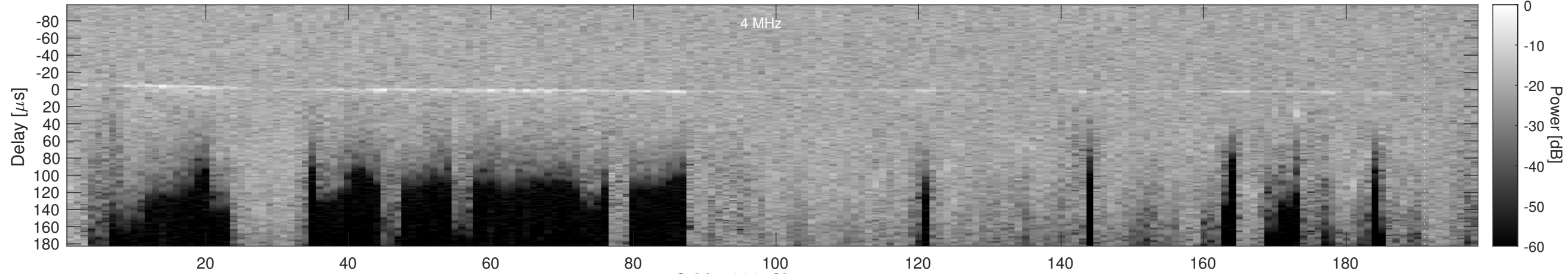
Orbit 4266, Cluttergram
