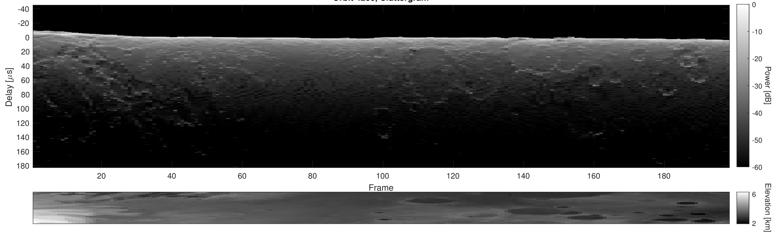
Orbit 4266, Cluttergram
