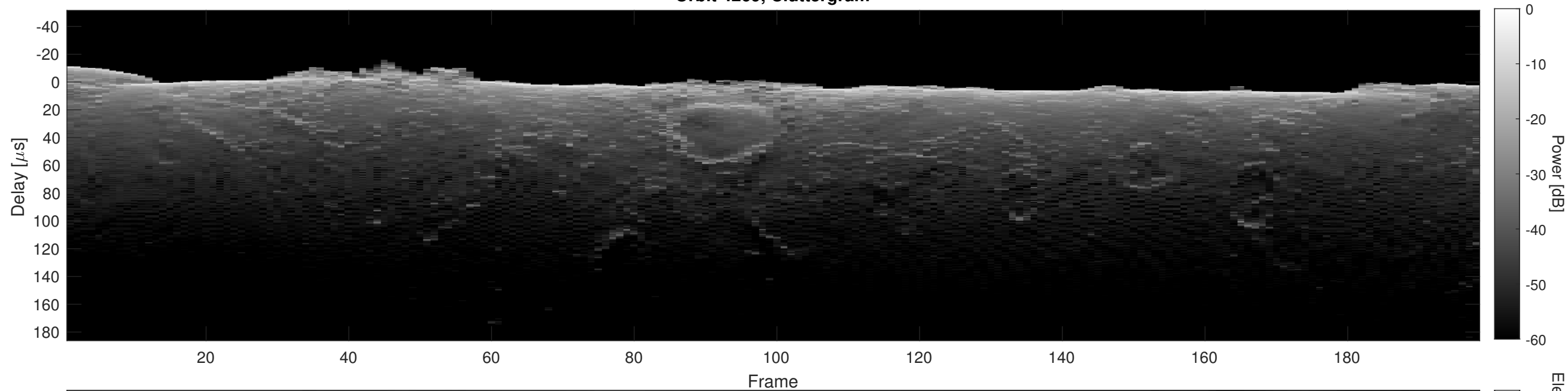
Orbit 4269, Cluttergram
