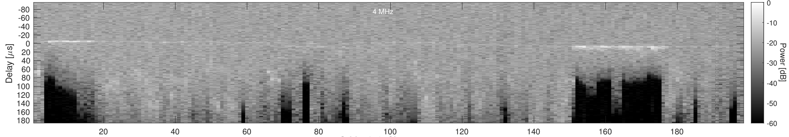
Orbit 4270, Cluttergram
