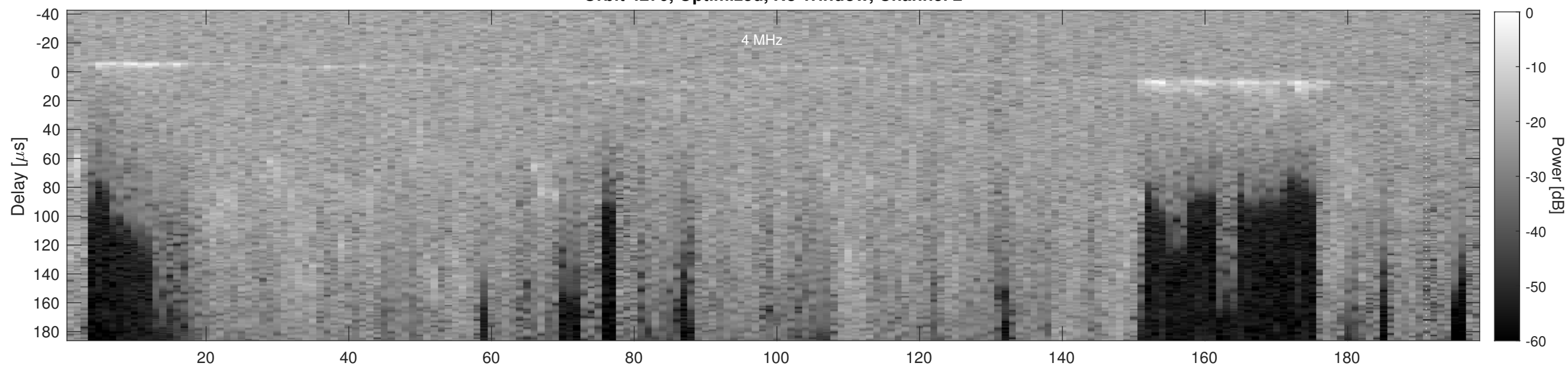
Orbit 4270, Cluttergram
