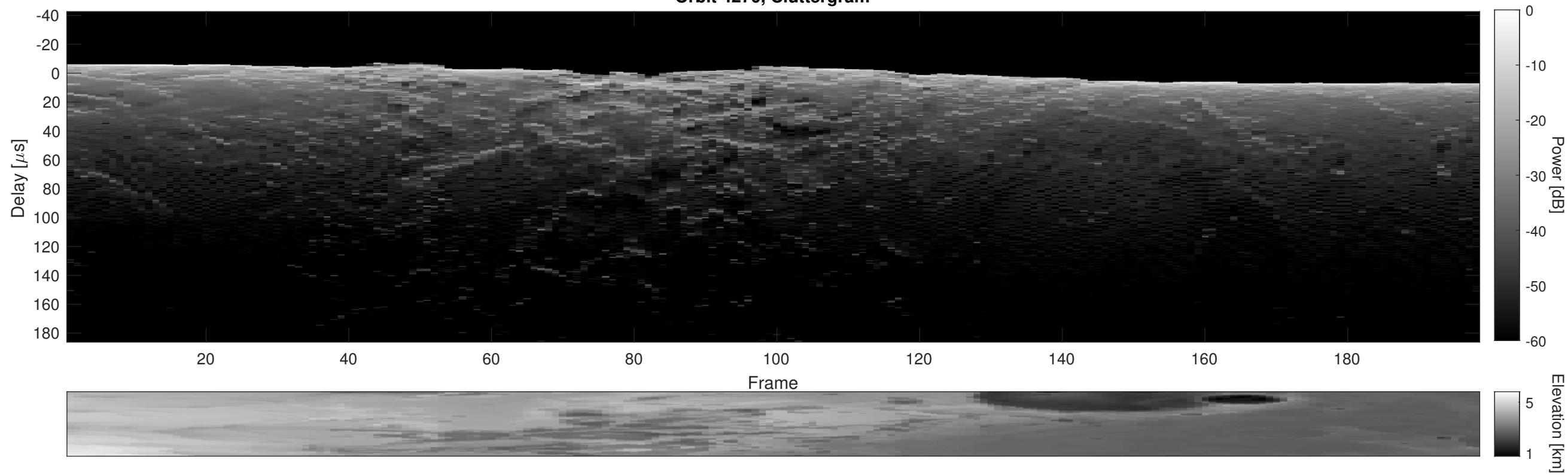
Orbit 4270, Cluttergram
