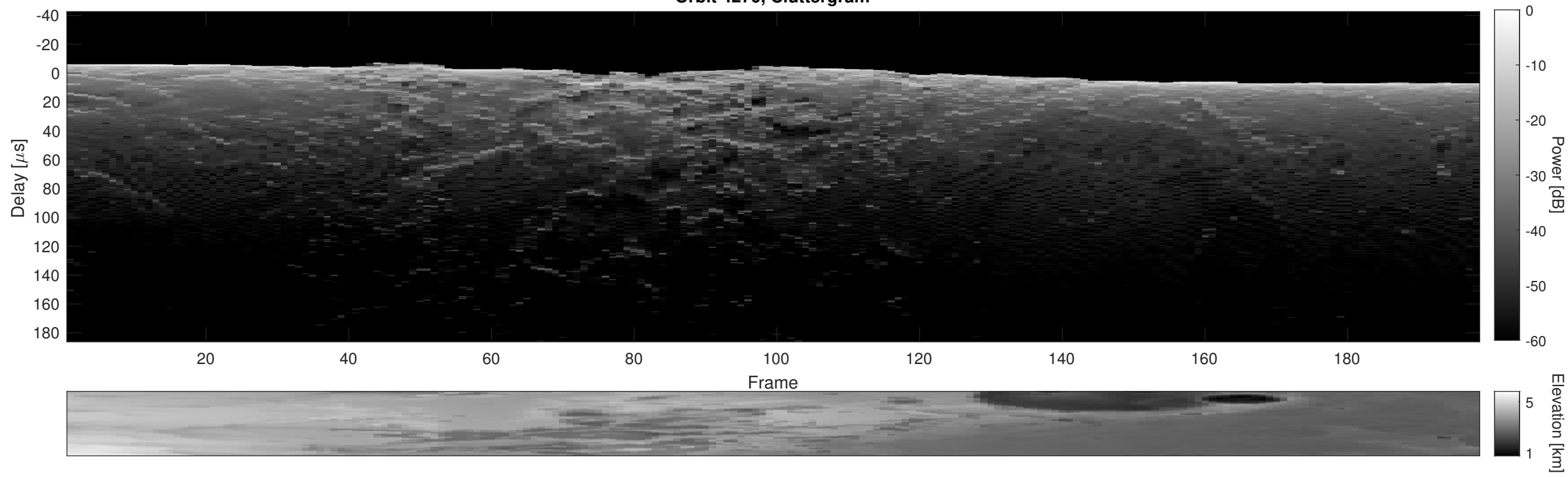
Orbit 4270, Cluttergram
