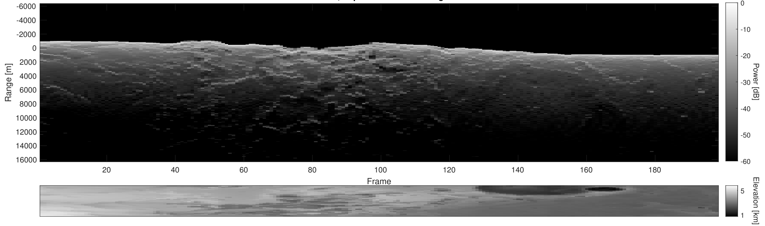
Orbit 4270, Depth-Corrected Cluttergram
