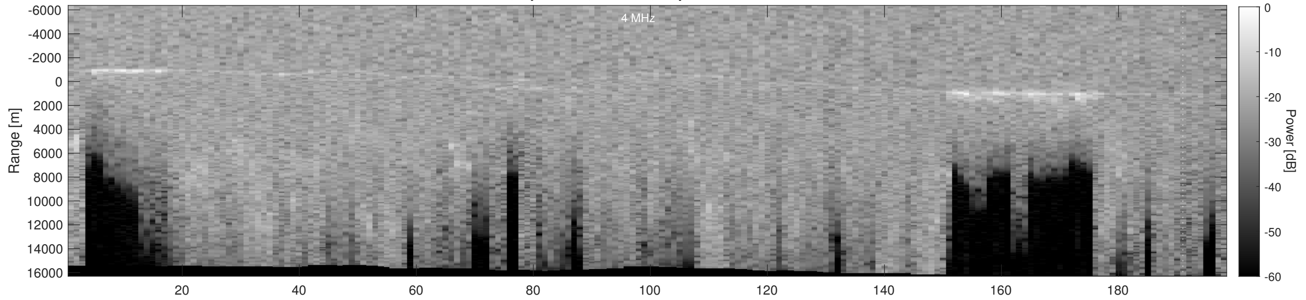
Orbit 4270, Depth-Corrected Cluttergram
