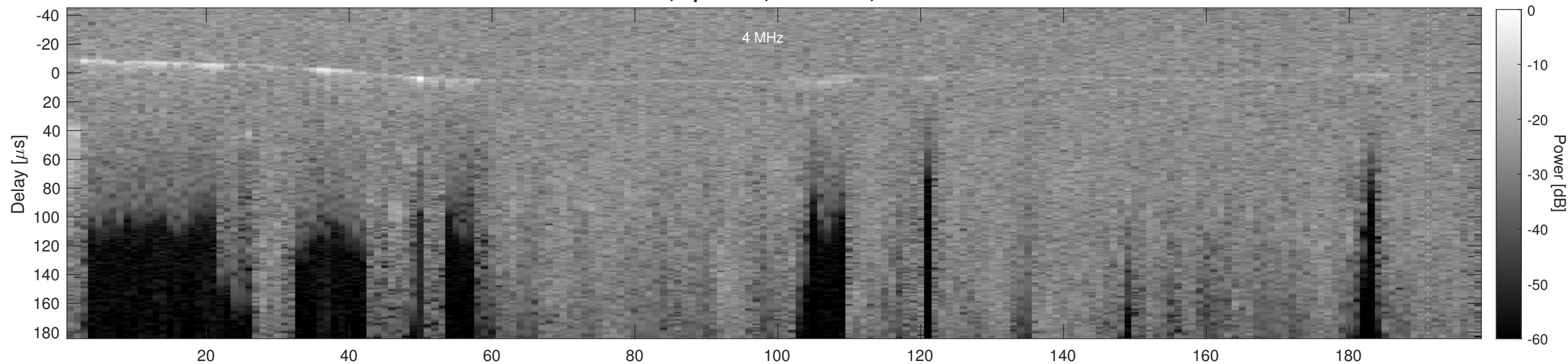
Orbit 4272, Cluttergram
