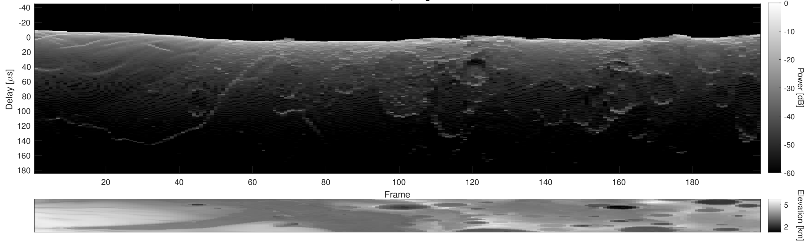
Orbit 4272, Cluttergram
