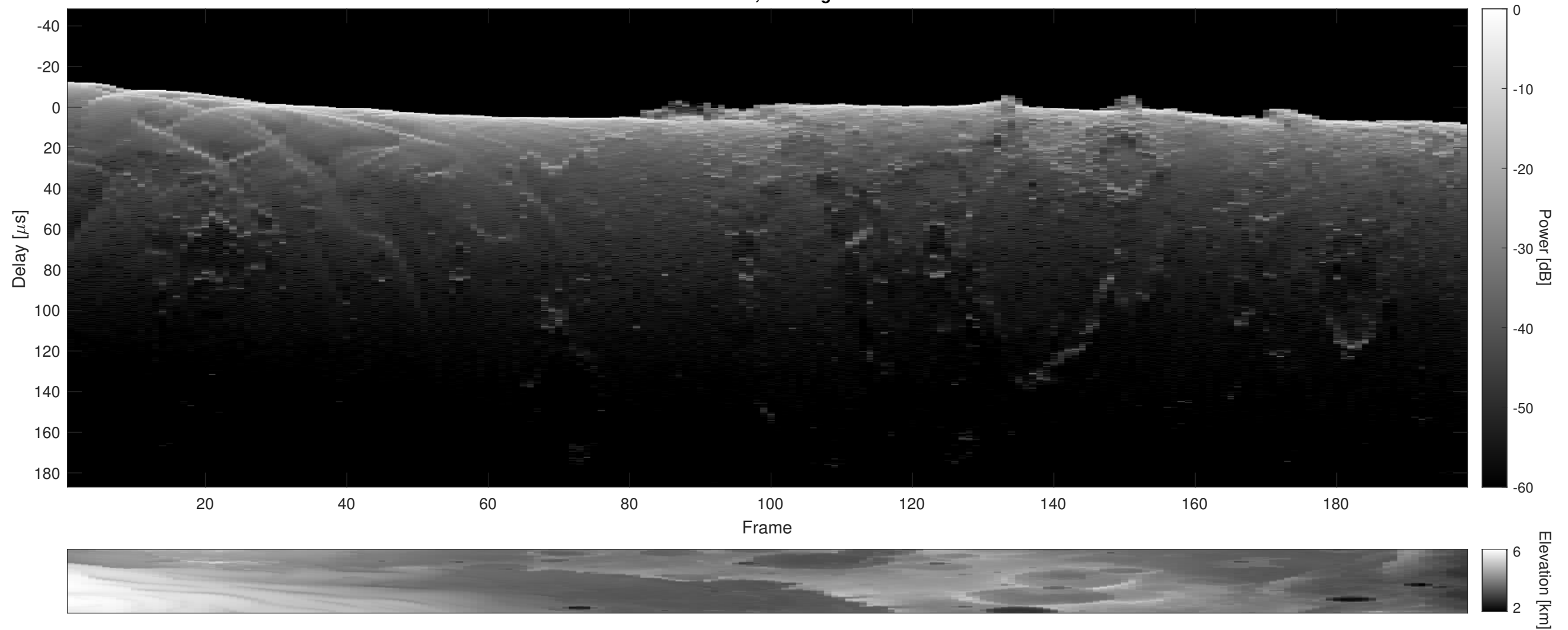
Orbit 4276, Cluttergram
