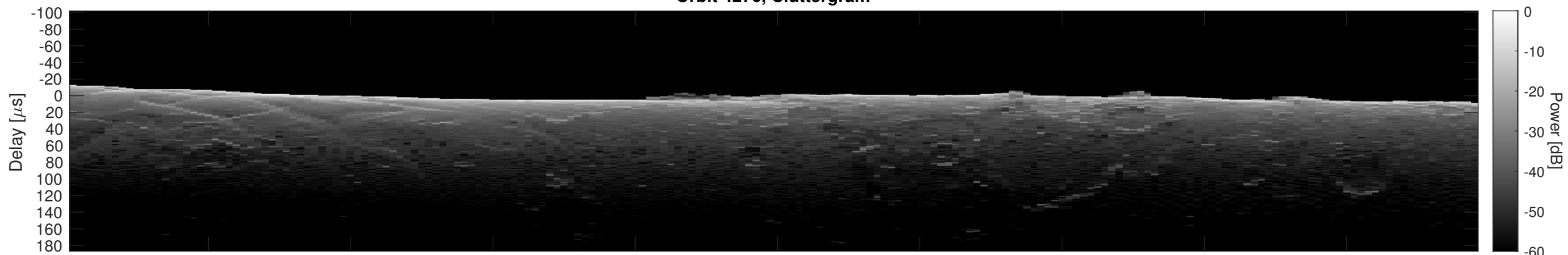
Orbit 4276, Cluttergram
