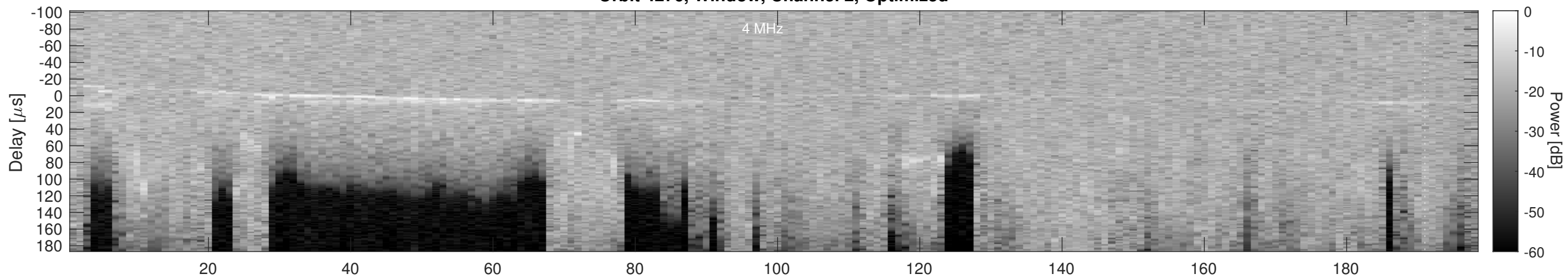
Orbit 4276, Cluttergram
