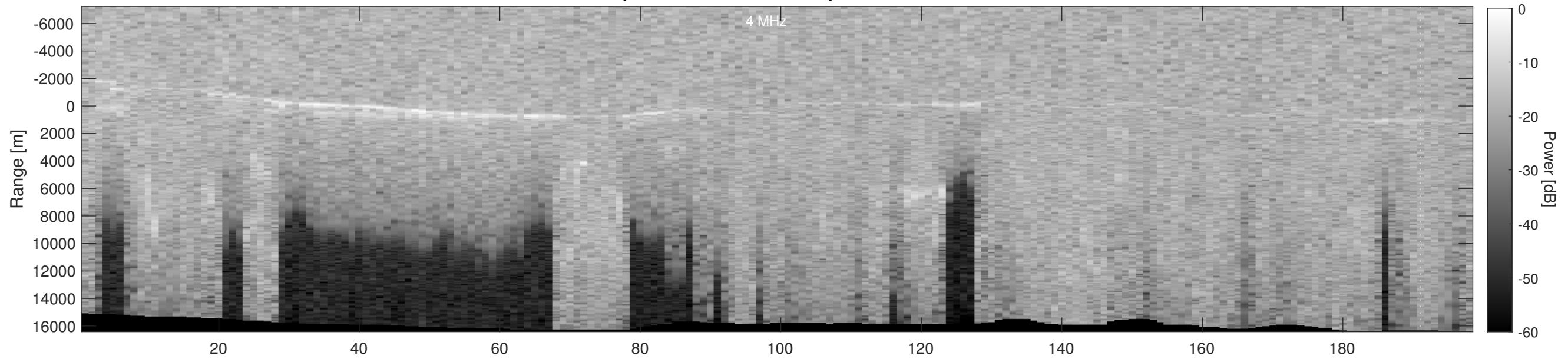
Orbit 4276, Depth-Corrected Cluttergram
