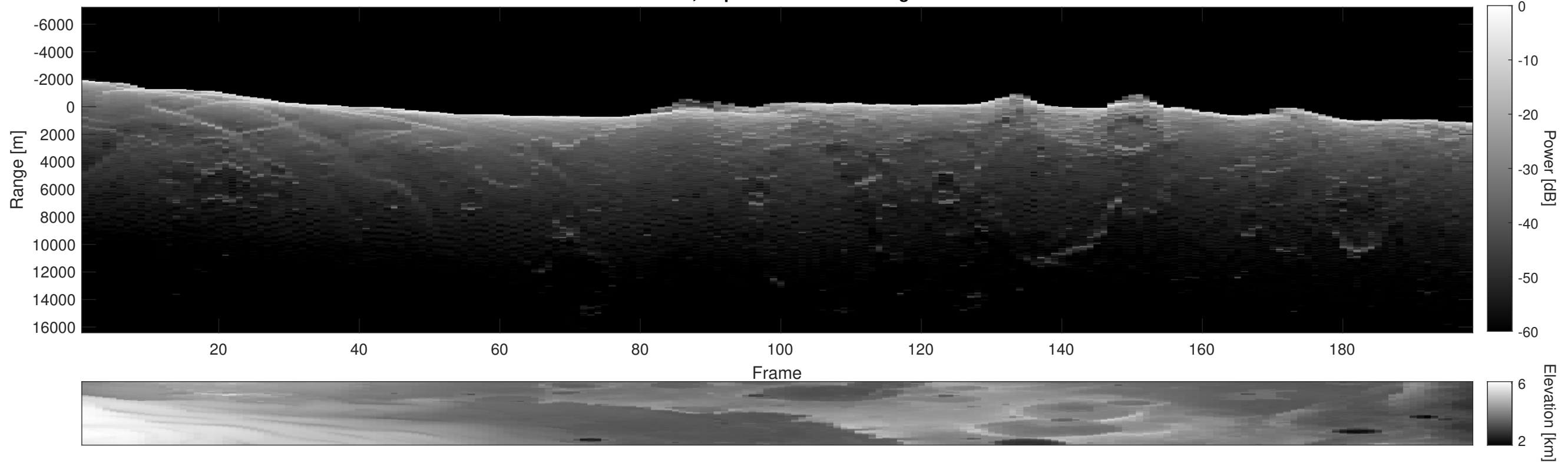
Orbit 4276, Depth-Corrected Cluttergram
