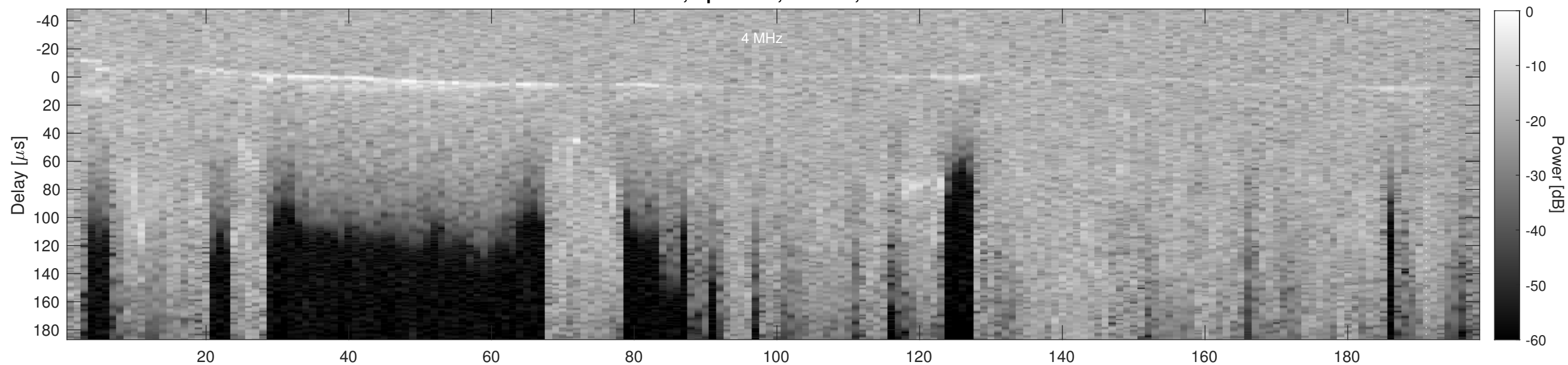
Orbit 4276, Cluttergram
