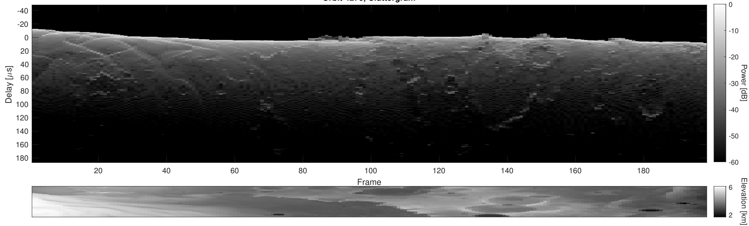
Orbit 4276, Cluttergram
