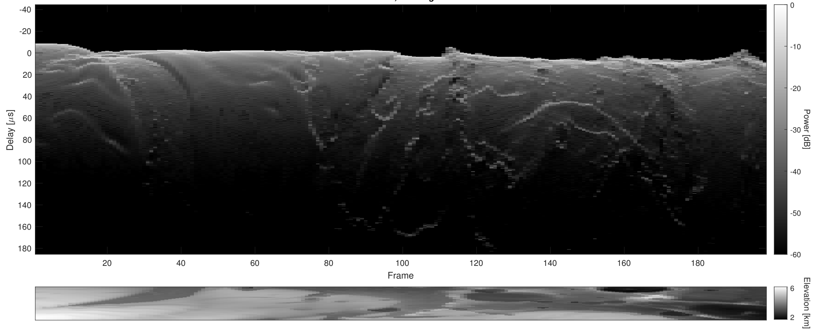
Orbit 4279, Cluttergram
