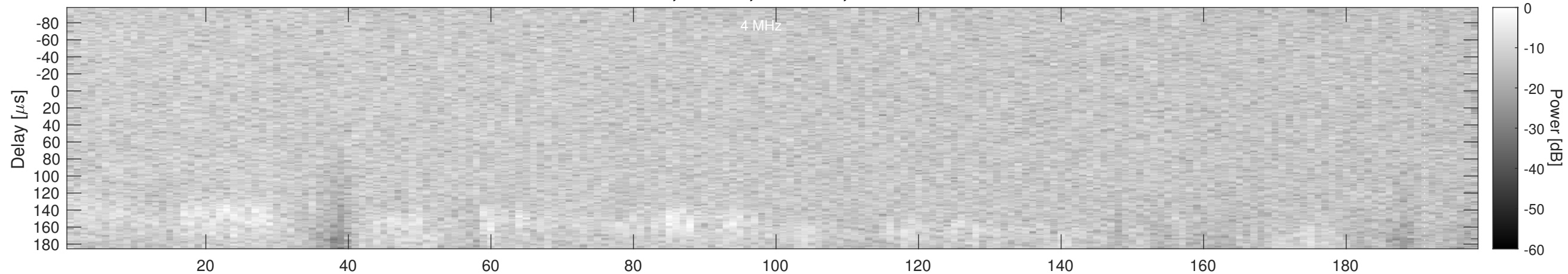
Orbit 4279, Window, Channel 2, Chapman
