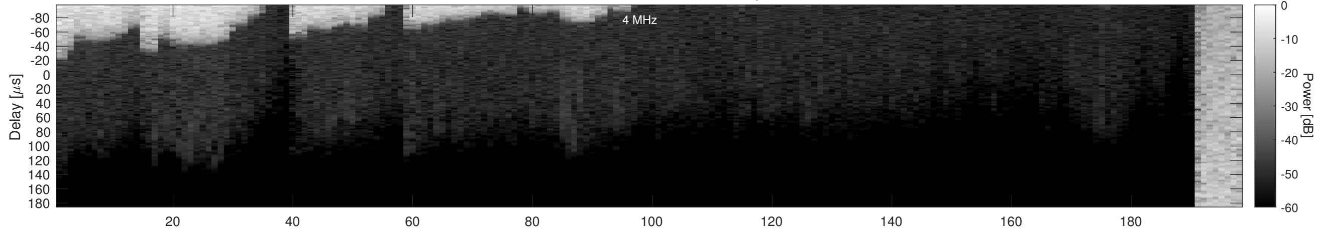
Orbit 4279, Window, Channel 2, Optimized
