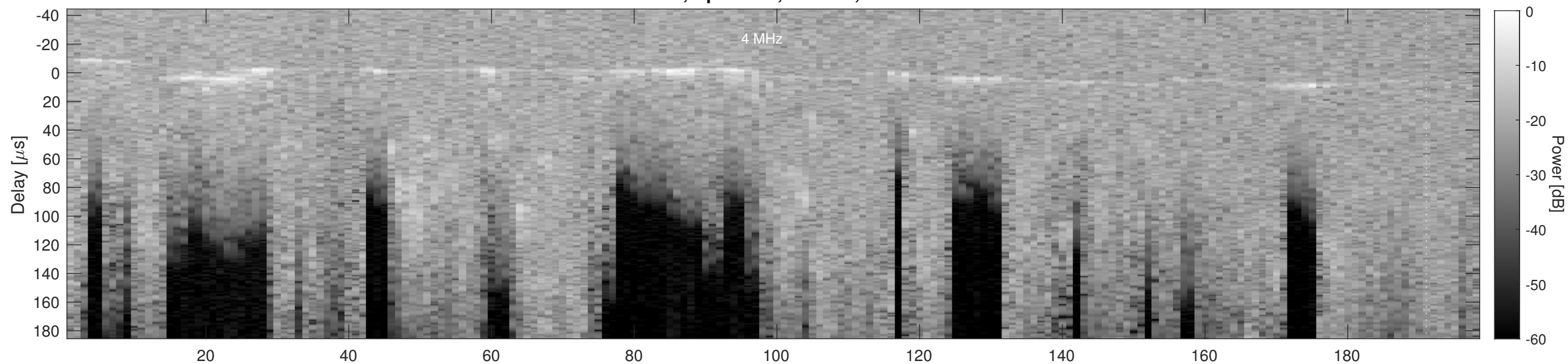
Orbit 4279, Cluttergram
