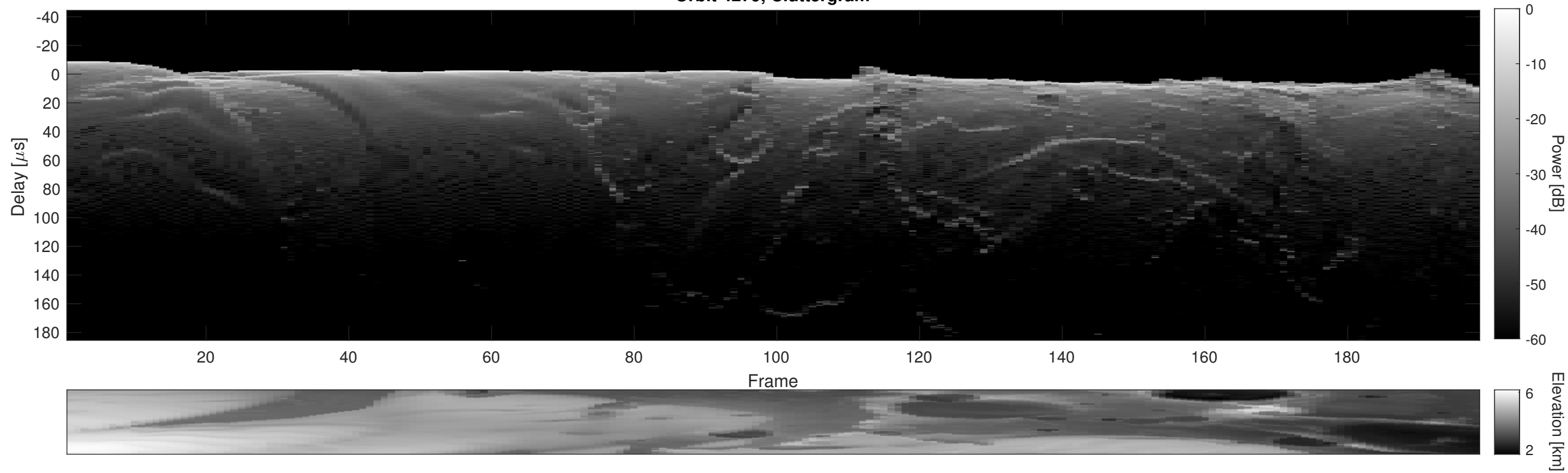
Orbit 4279, Cluttergram
