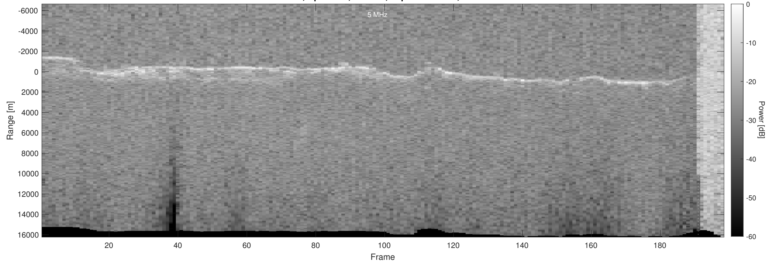
Orbit 4279, Optimized, Window, Depth-Corrected, Channel 2
