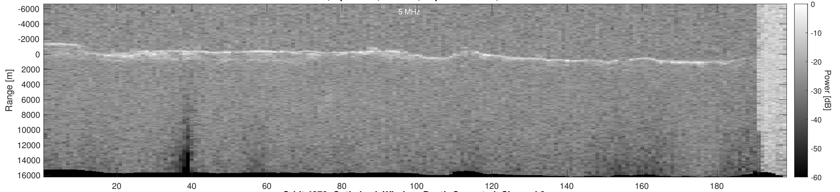
Orbit 4279, Optimized, Window, Depth-Corrected, Channel 2
