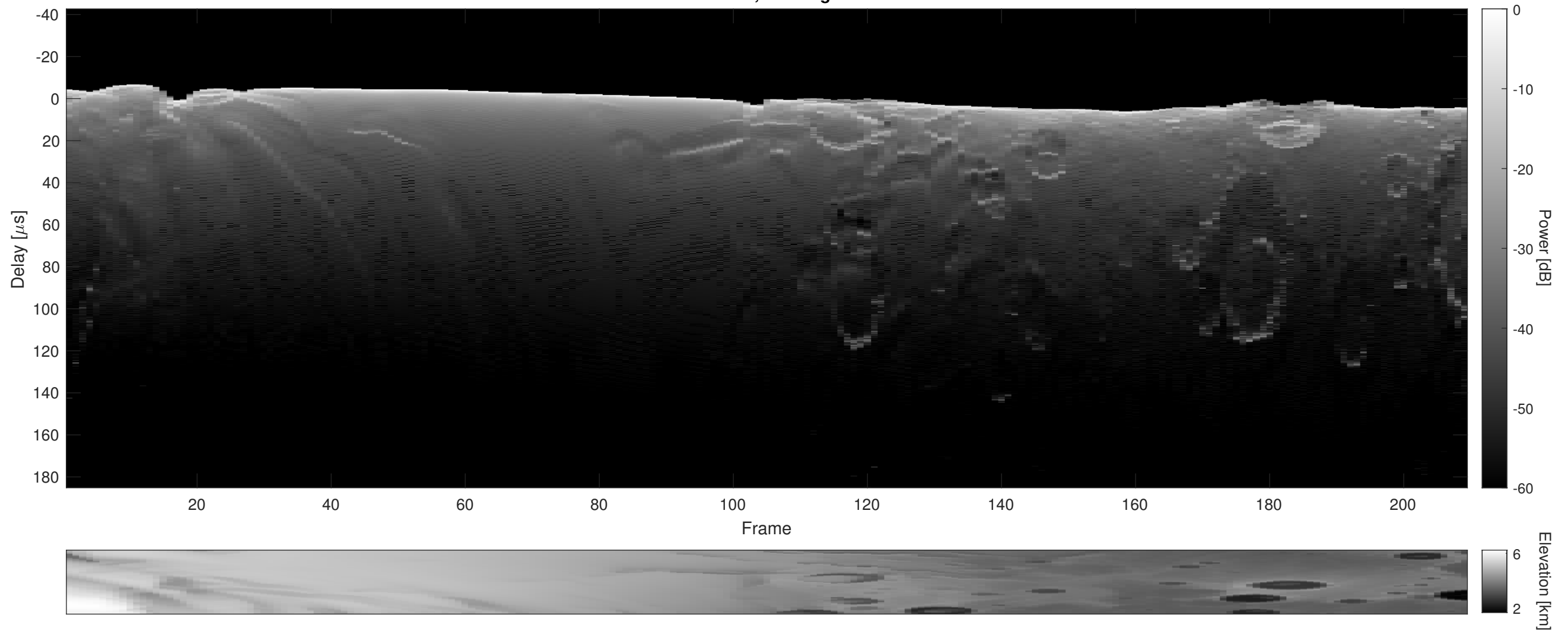
Orbit 4289, Cluttergram
