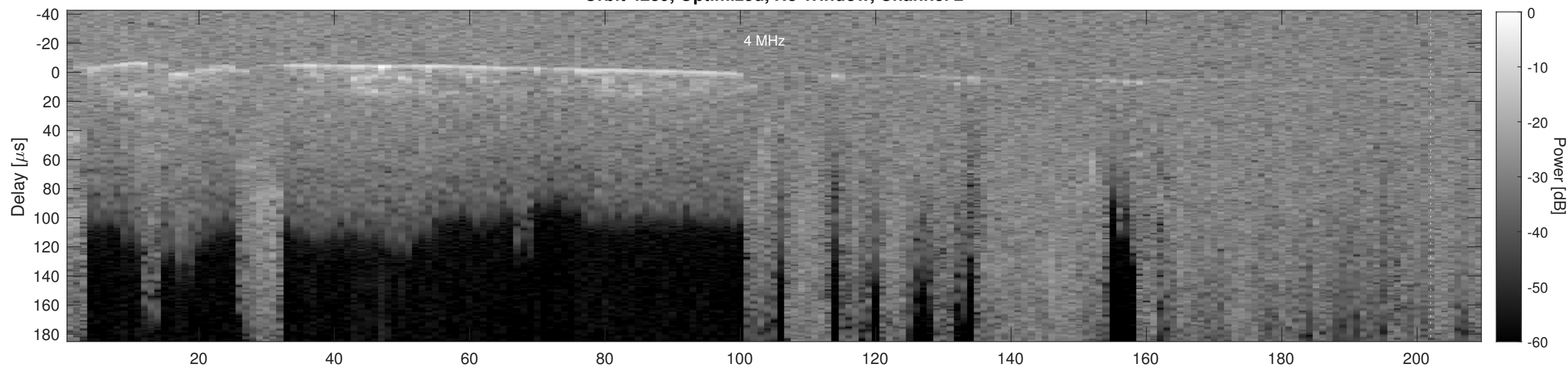
Orbit 4289, Cluttergram
