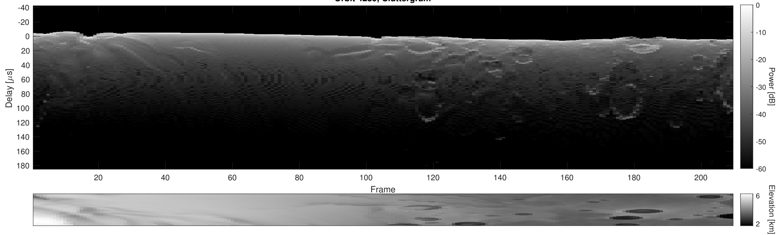
Orbit 4289, Cluttergram
