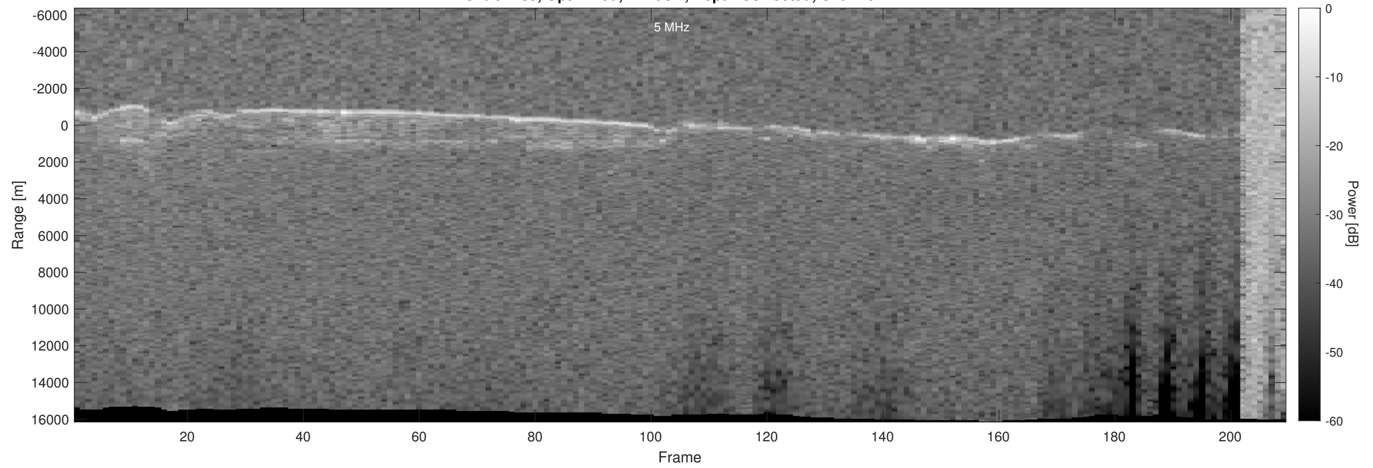
Orbit 4289, Optimized, Window, Depth-Corrected, Channel 2
