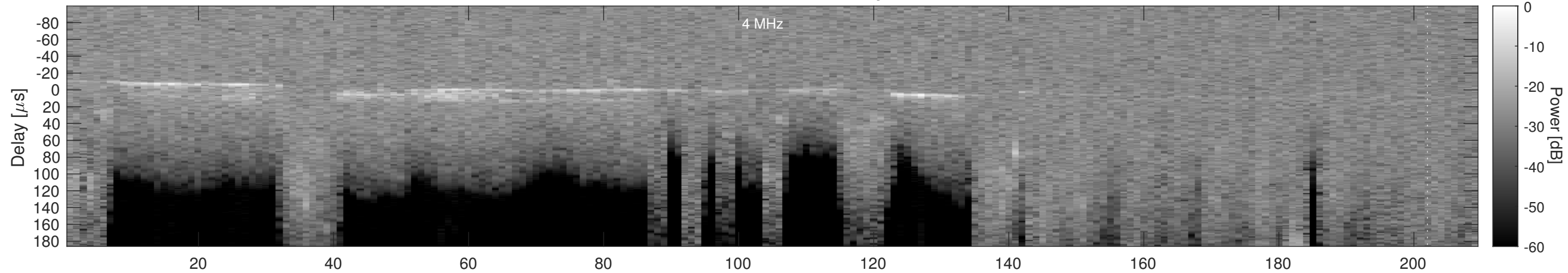
Orbit 4290, Cluttergram
