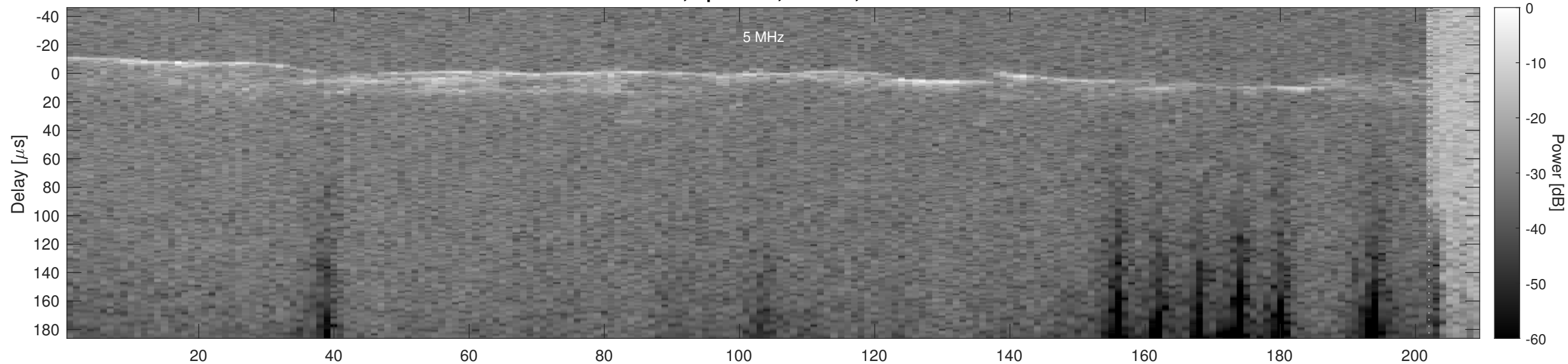
Orbit 4290, Optimized, Window, Channel 2
