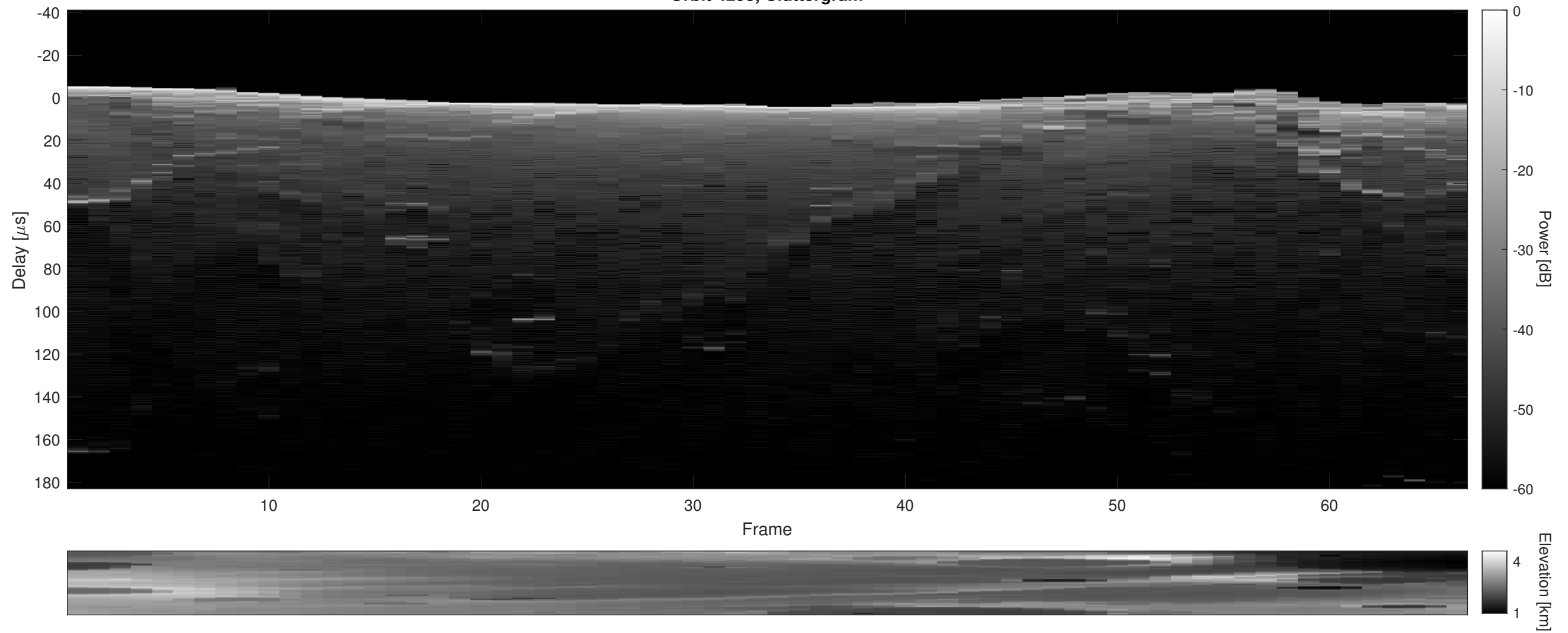
Orbit 4293, Cluttergram
