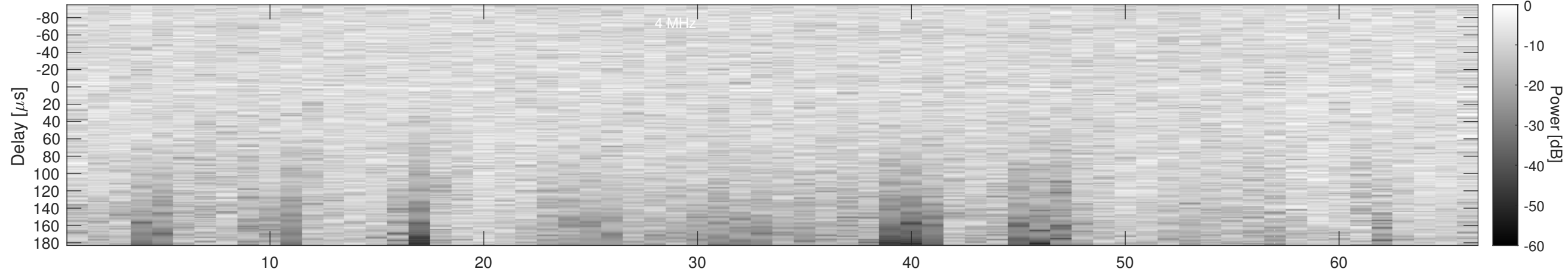
Orbit 4293, Cluttergram
