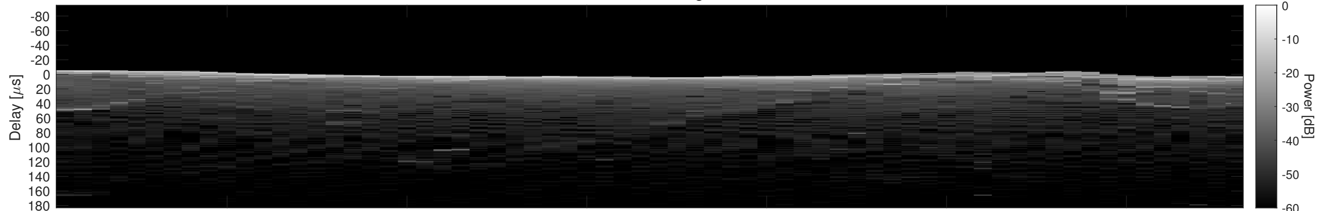
Orbit 4293, Cluttergram
