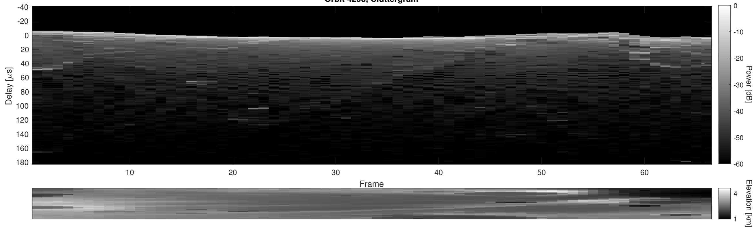
Orbit 4293, Cluttergram
