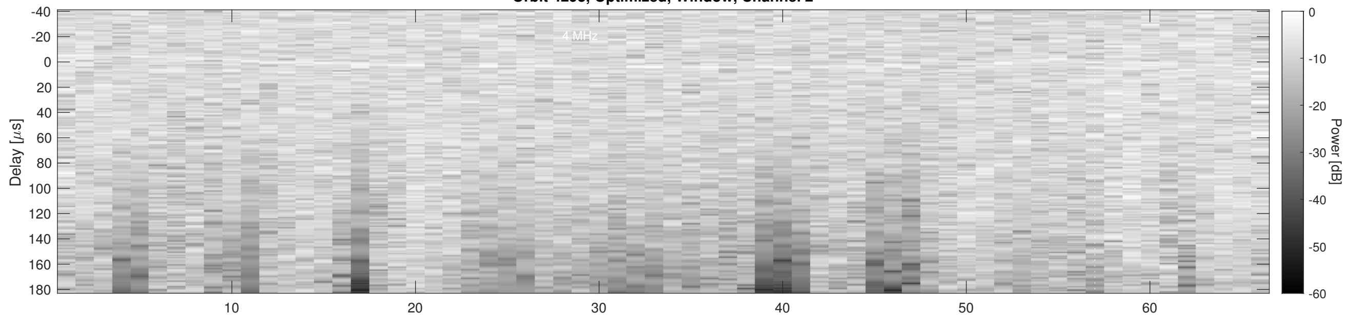
Orbit 4293, Cluttergram
