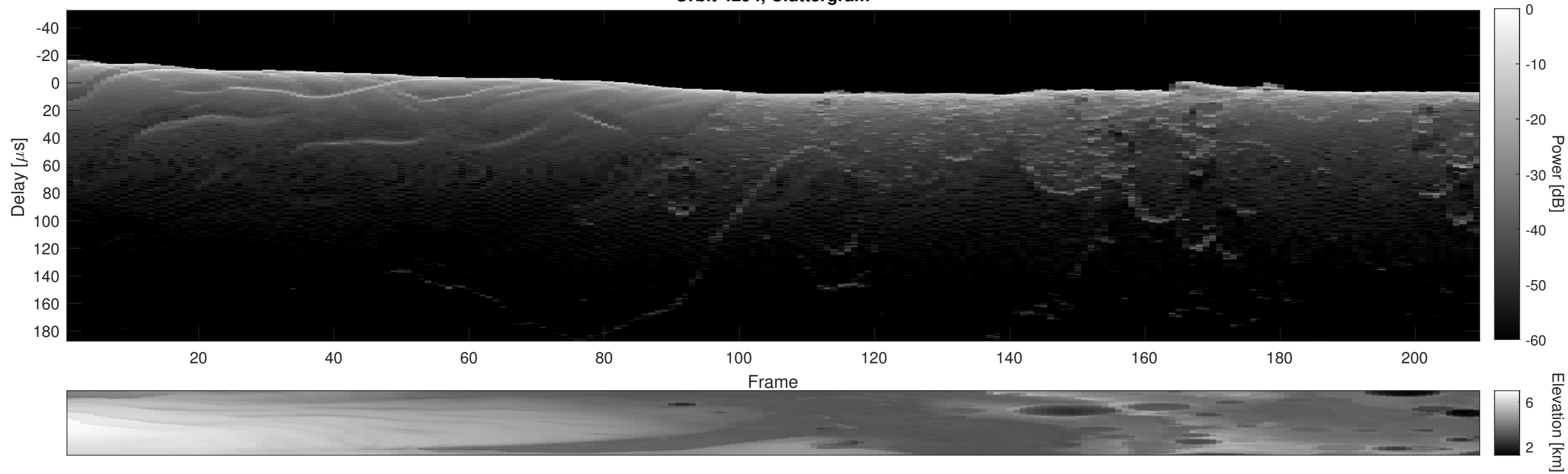
Orbit 4294, Cluttergram
