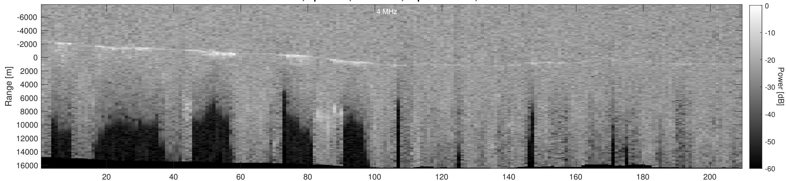
Orbit 4294, Depth-Corrected Cluttergram
