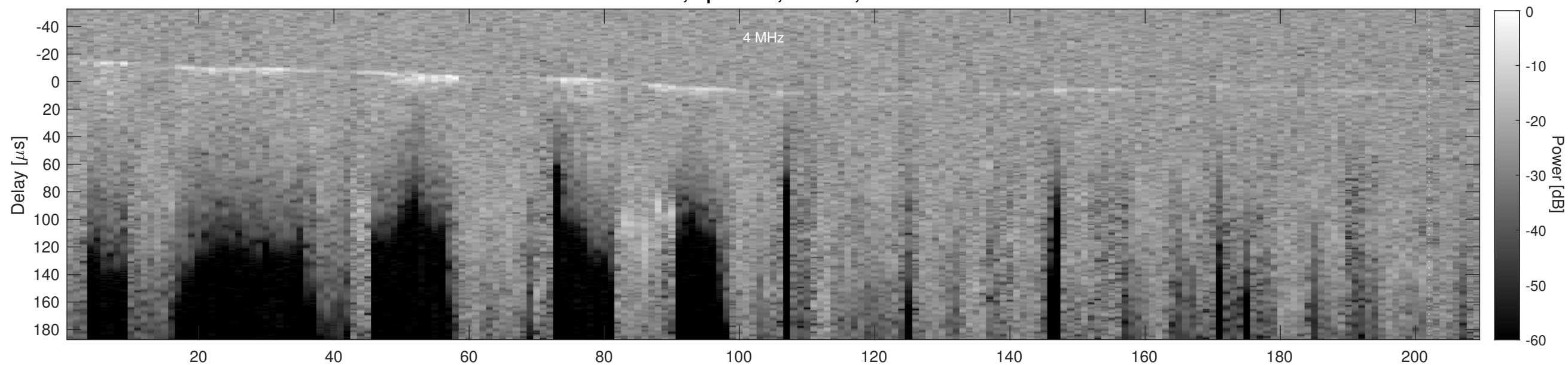
Orbit 4294, Cluttergram
