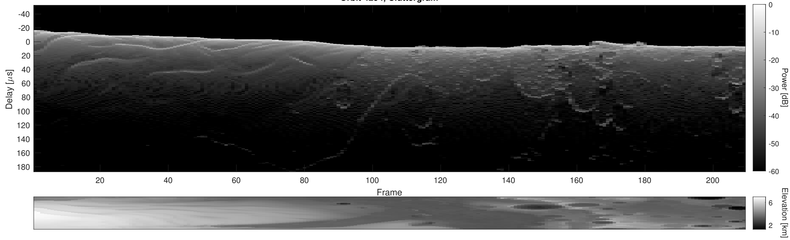
Orbit 4294, Cluttergram
