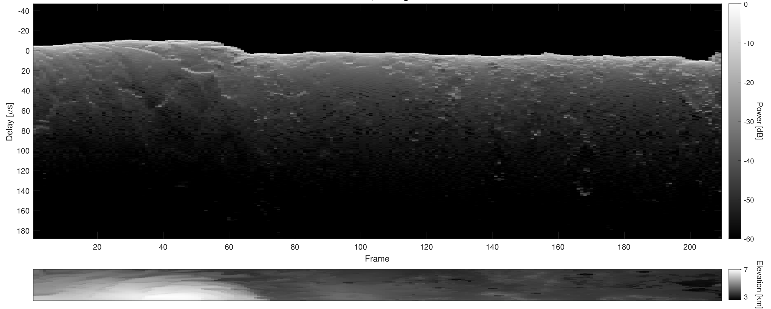
Orbit 4295, Cluttergram
