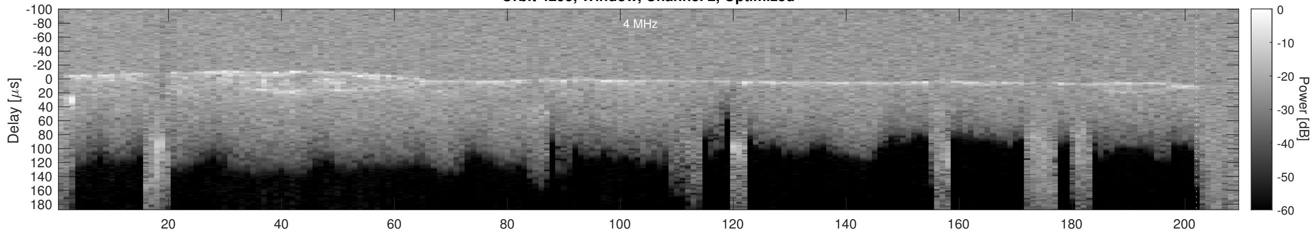
Orbit 4295, Cluttergram
