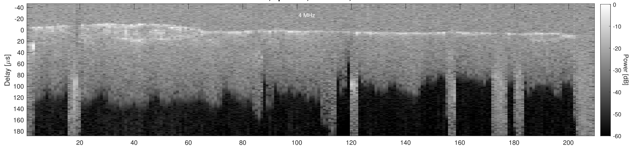
Orbit 4295, Cluttergram
