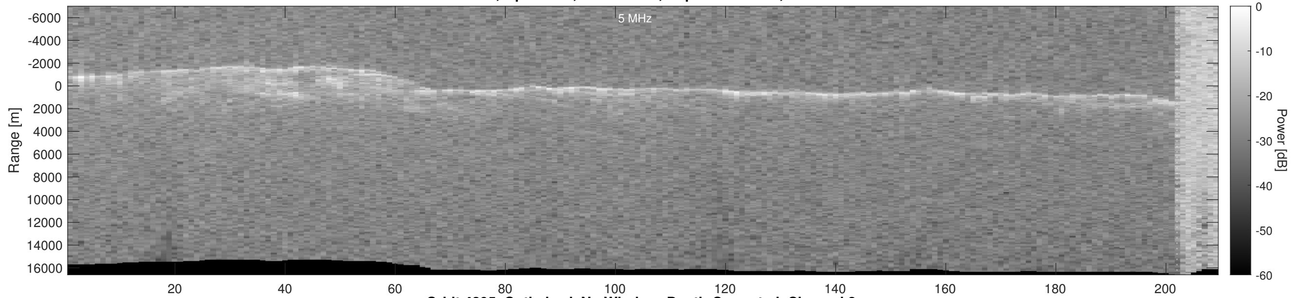
Orbit 4295, Optimized, No Window, Depth-Corrected, Channel 2
