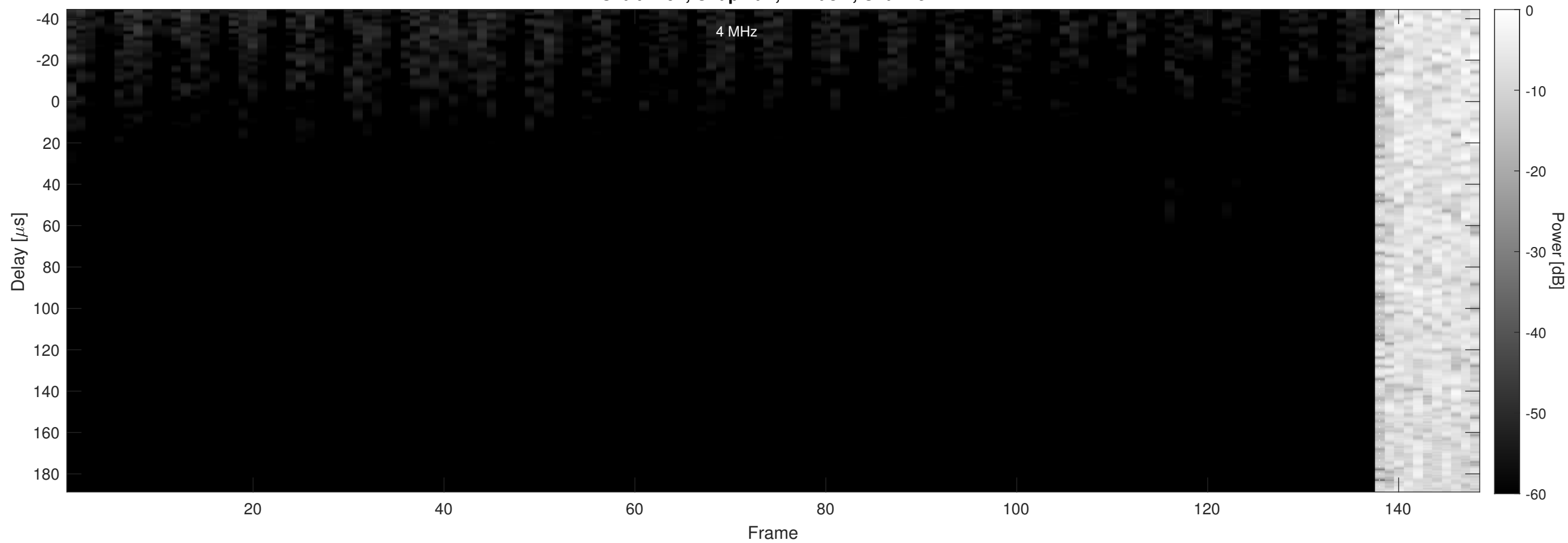
Orbit 4297, Chapman, Window, Channel 2
